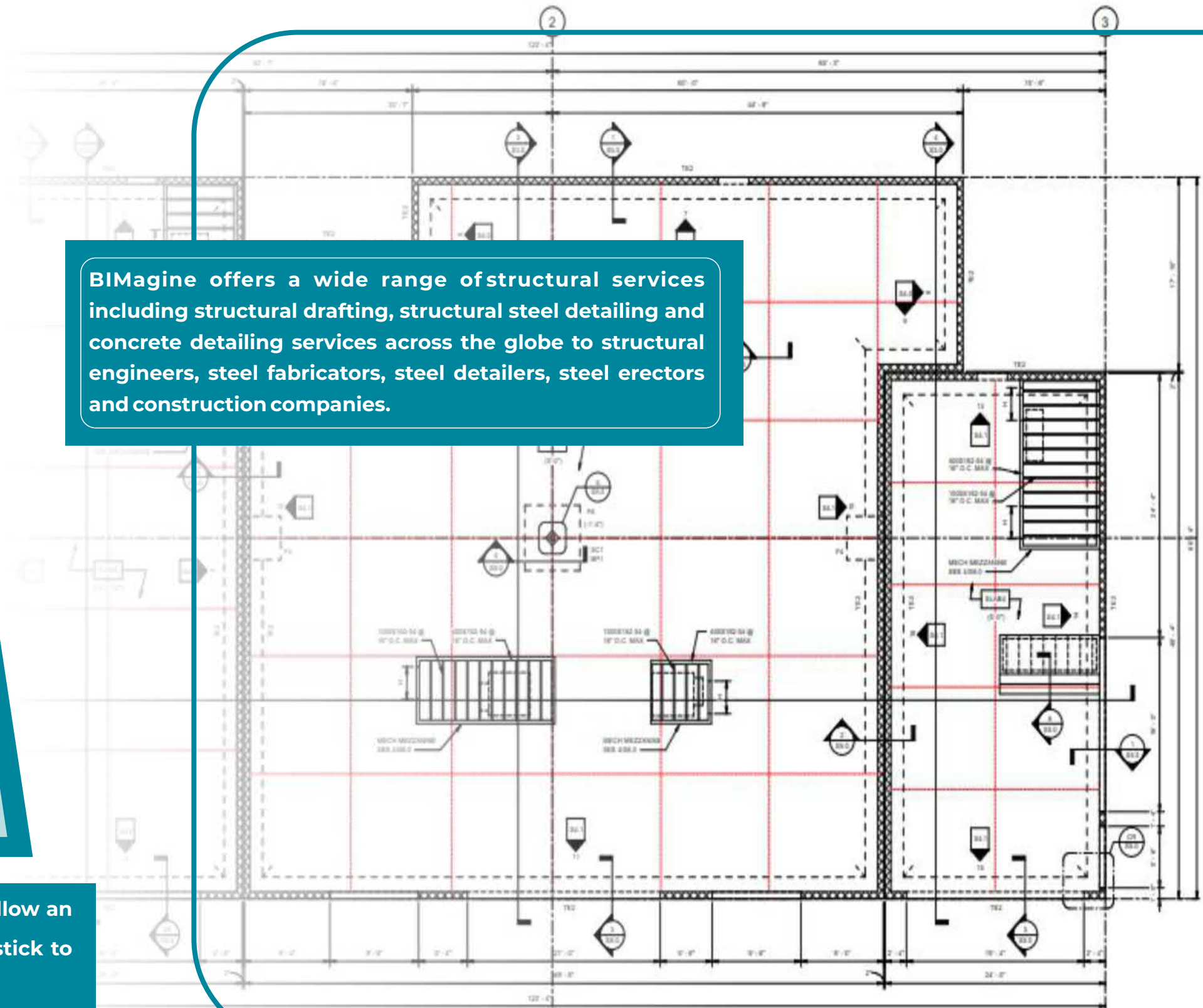
Foundation Plan
