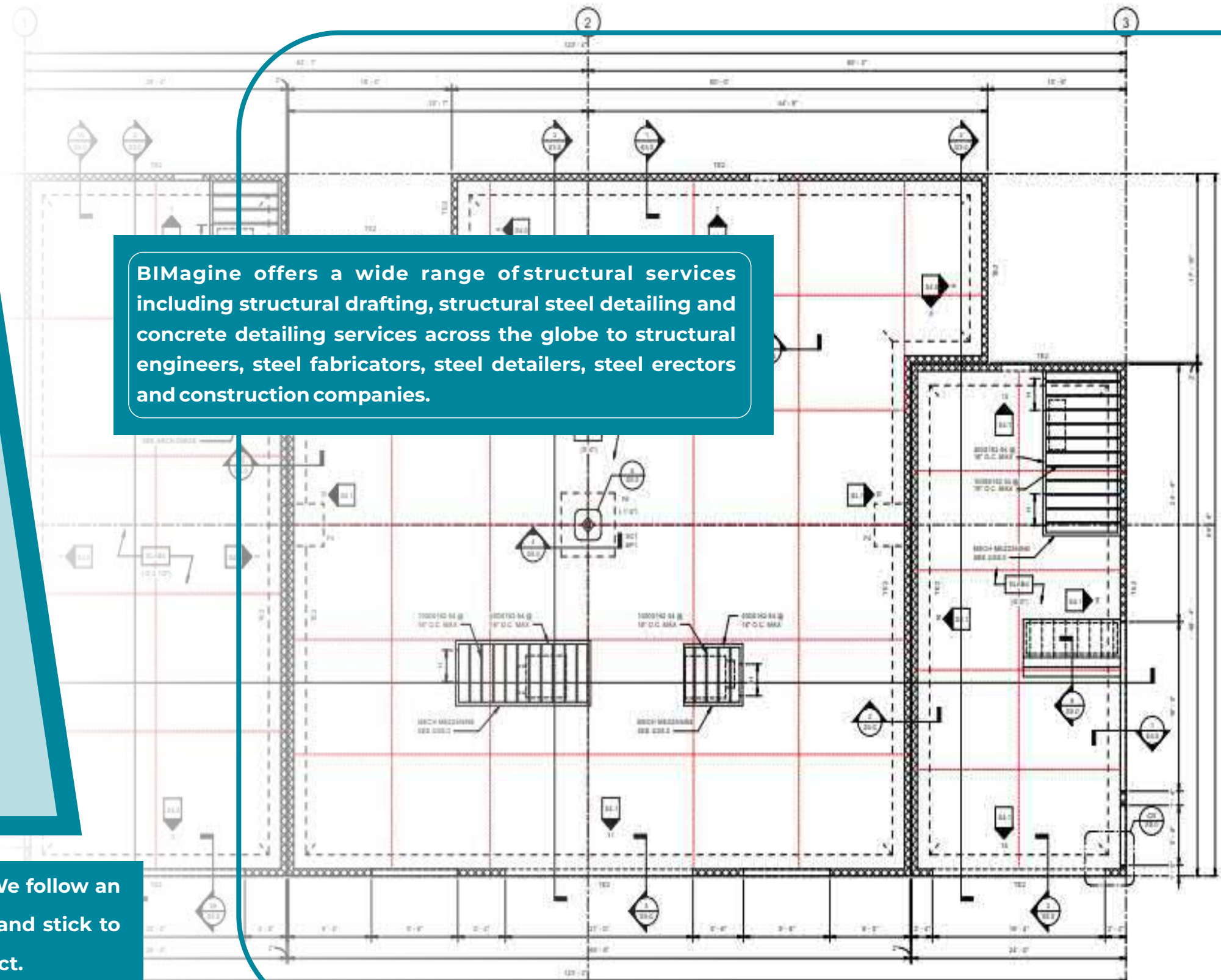
Foundation Plan
