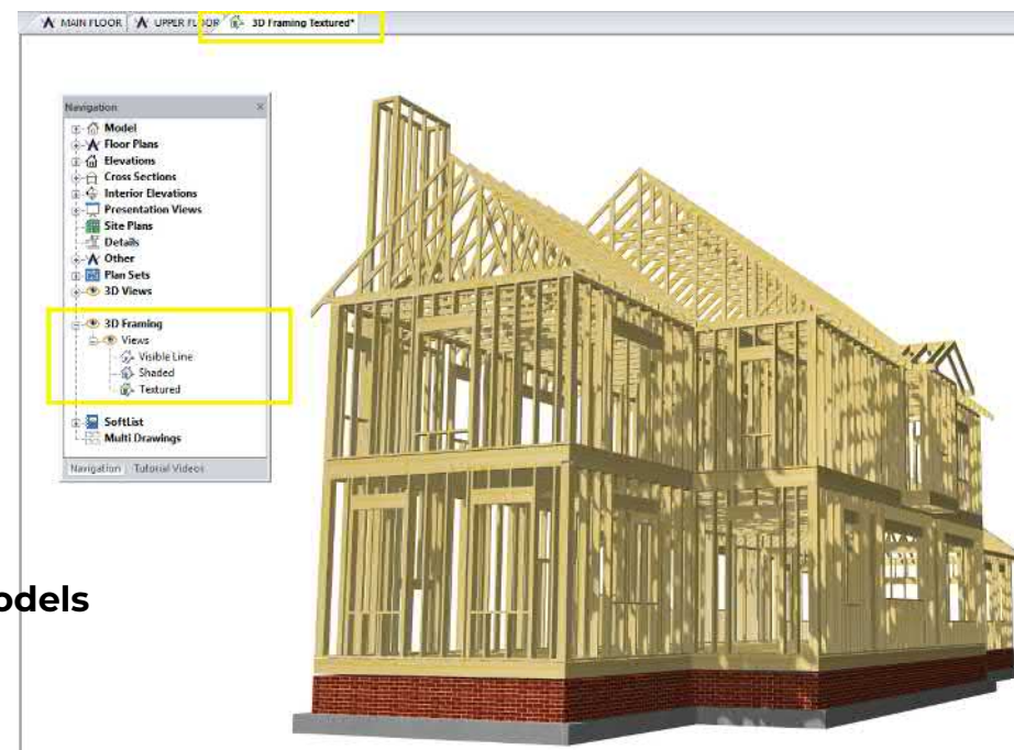
Wooden Structural BIM Modeling
